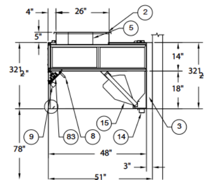
Z-SCRUB ZST-40 SIDE VIEW
