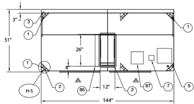
Z-SCRUB ZST-40 TOP VIEW
