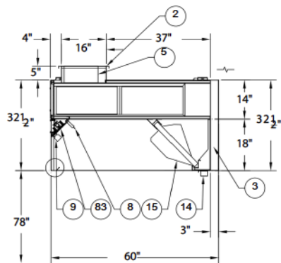
Z-SCRUB ZST-20 SIDE VIEW
