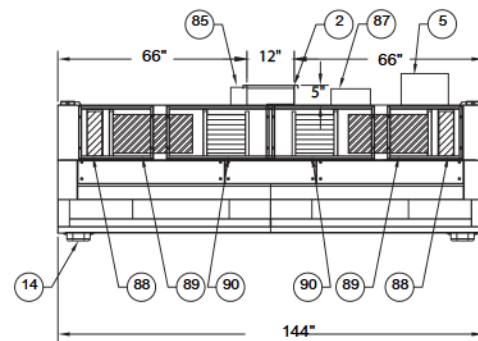
Z-SCRUB ZST-40 FRONT VIEW
