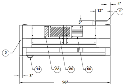
Z-SCRUB ZST-20 FRONT VIEW
