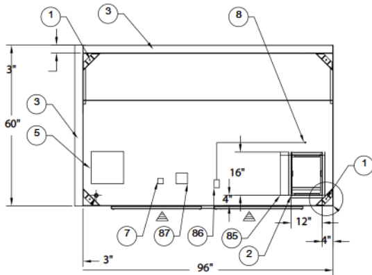
Z-SCRUB ZST-20 TOP VIEW
