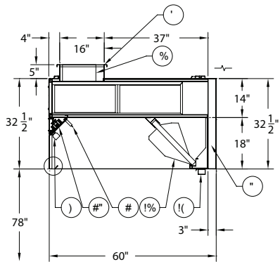
Z-scrub ZST-20-T SIDE VIEW
