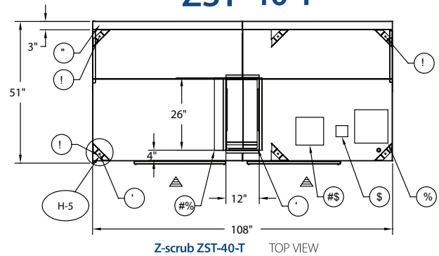
Z-scrub ZST-40-T TOP VIEW
