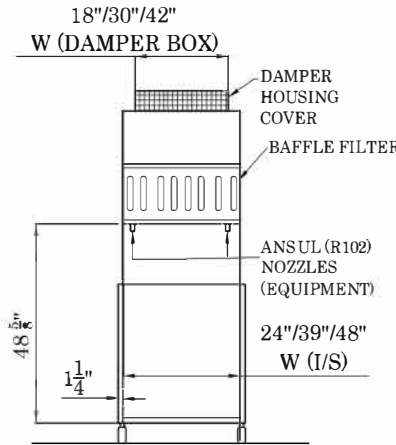
RIGHT SIDE ELEVATION VIEW
