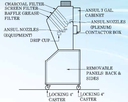
RIGHT SIDE ELEVATION VIEW
