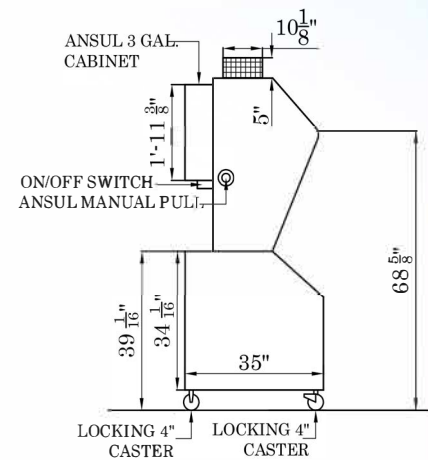
LEFT SIDE ELEVATION VIEW
